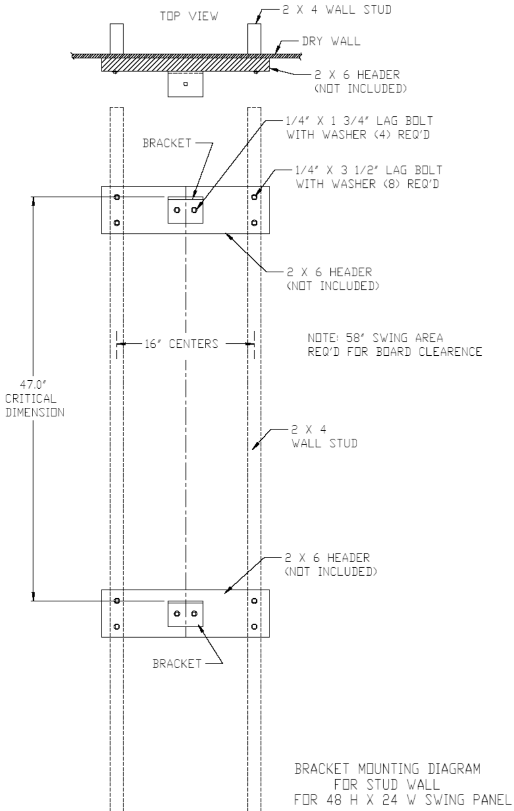
FIGURE 1-4 HEADER INSTALLATION
